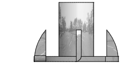
(54) BG - T-NUT 5/16 - H100074
